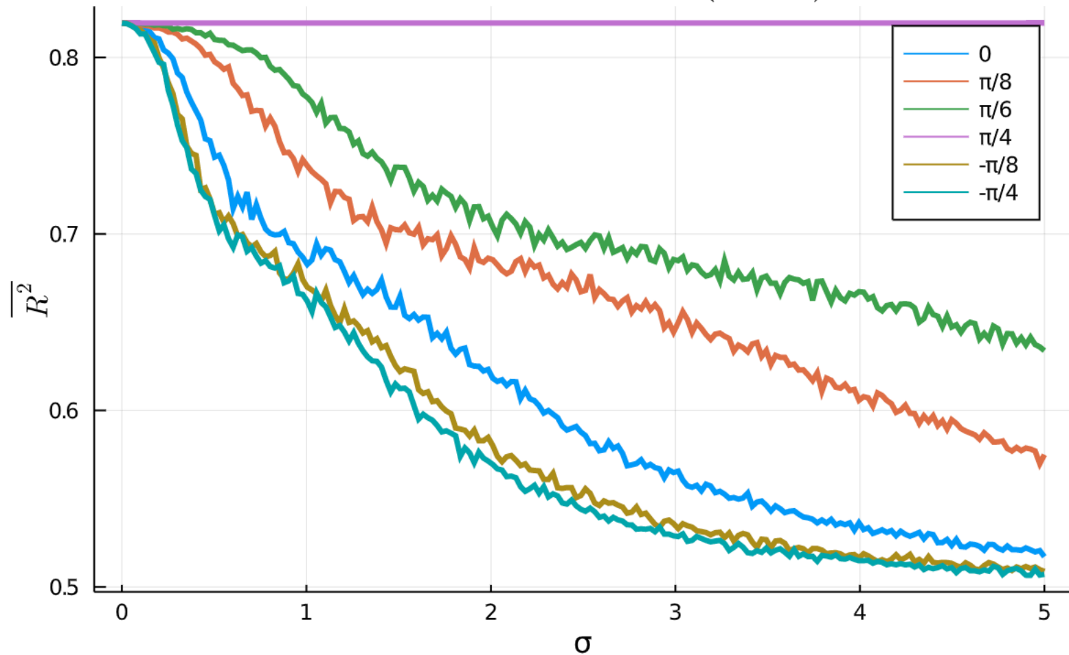
\overline{R^2} vs. \sigma for Several \theta ( k=1.3 )
